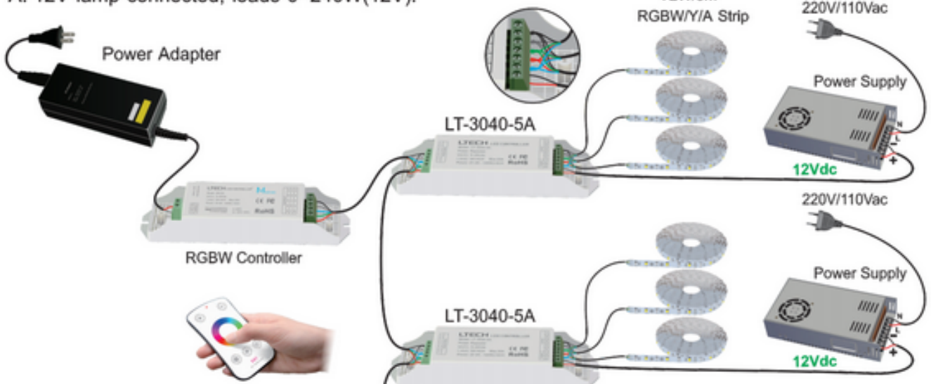
A. 12V lamp connected, loads 0~240W(12V).
